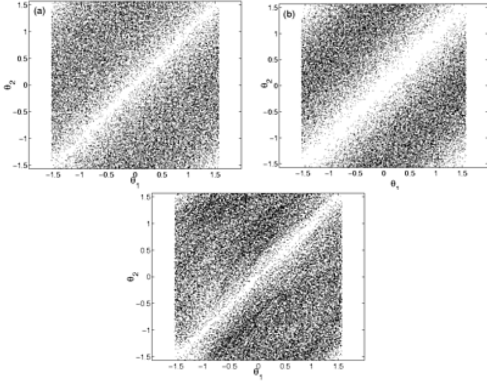
FIG. 1: (a) Scatter plot of \theta_1 vs \theta_2 , in the TRS case. (b) Scatter plot of \theta_1 vs \theta_2 in the TRSB case. (c) Scatter plot of \theta_1 vs \theta_2 from the HFSS simulation, with 100 realizations and sweeping frequency from 6.75GHz to 8.75GHz.
