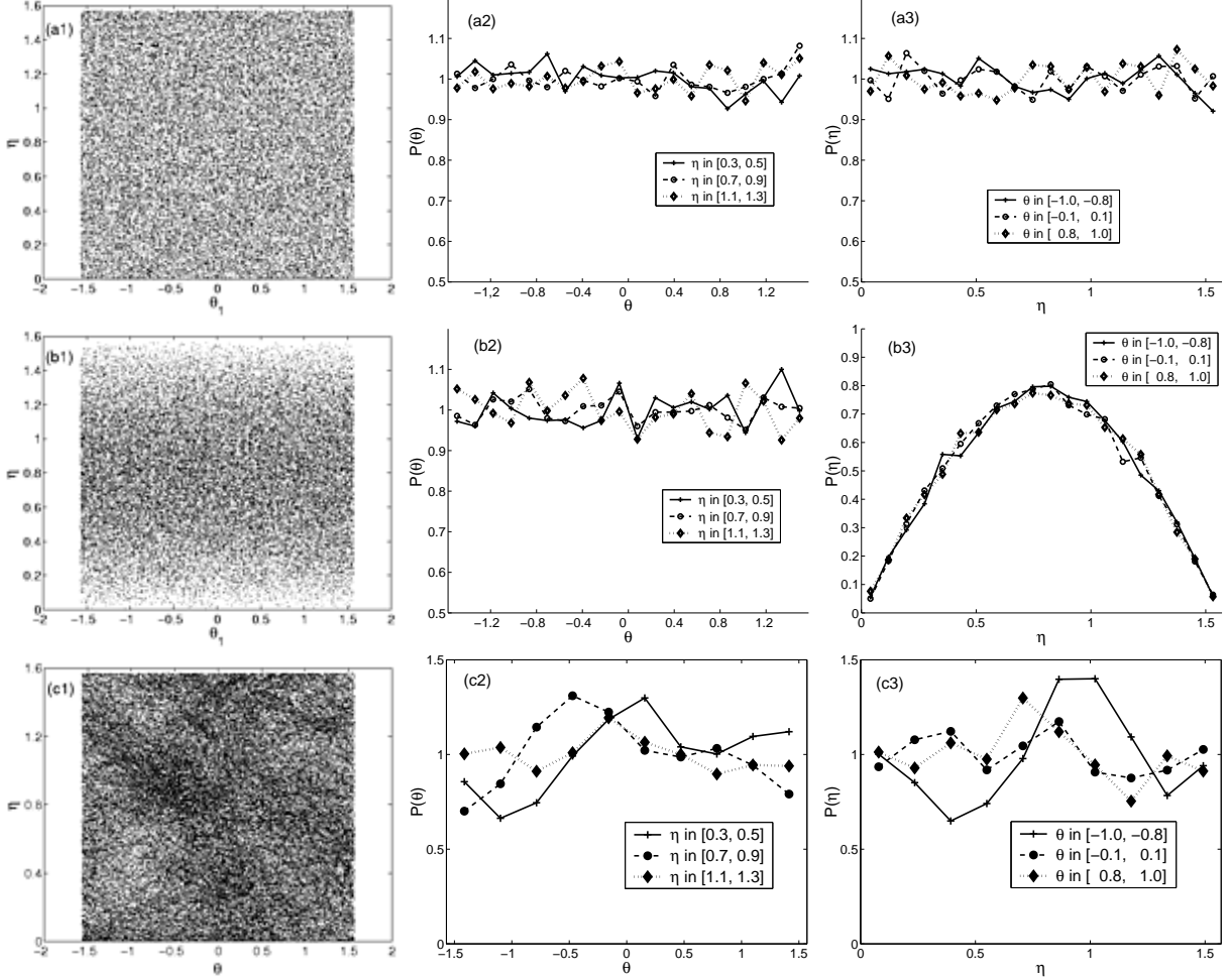
FIG. 2: Scatter plot of \eta vs \theta for (a1) the model impedance in the TRS case, (b1) the model impedance in the TRSB case, and (c1) from the HFSS simulation. Plots (a2) and (a3) [(b2) and (b3), (c2) and (c3)] show conditional probability for \theta and for \eta for the model TRS case [model TRSB case, the HFSS simulation].
