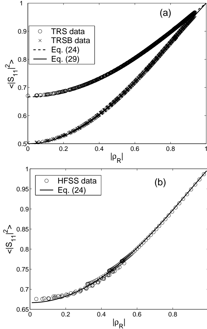
FIG. 3: (a) Numerical simulation for the average reflection coefficient \langle |S_{11}|^2 \rangle vs magnitude of \rho_R defined in Eq. (25) for the TRS and the TRSB system, taking 10^6 realization of the impedance matrix, 30 uniformly spaced values of \gamma_R from 0.1 to 3, and 31 equally spaced values of \gamma_X from 0 to 3. (b) Average reflection coefficient \langle |S_{11}|^2 \rangle vs |\rho_R| using the cavity impedance and radiation impedance from HFSS calculation and varying the values of Z_0 and the capacitive reactance Y
